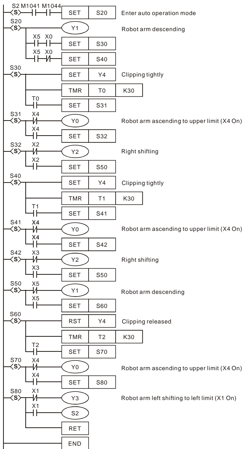
Ladder Diagram:
