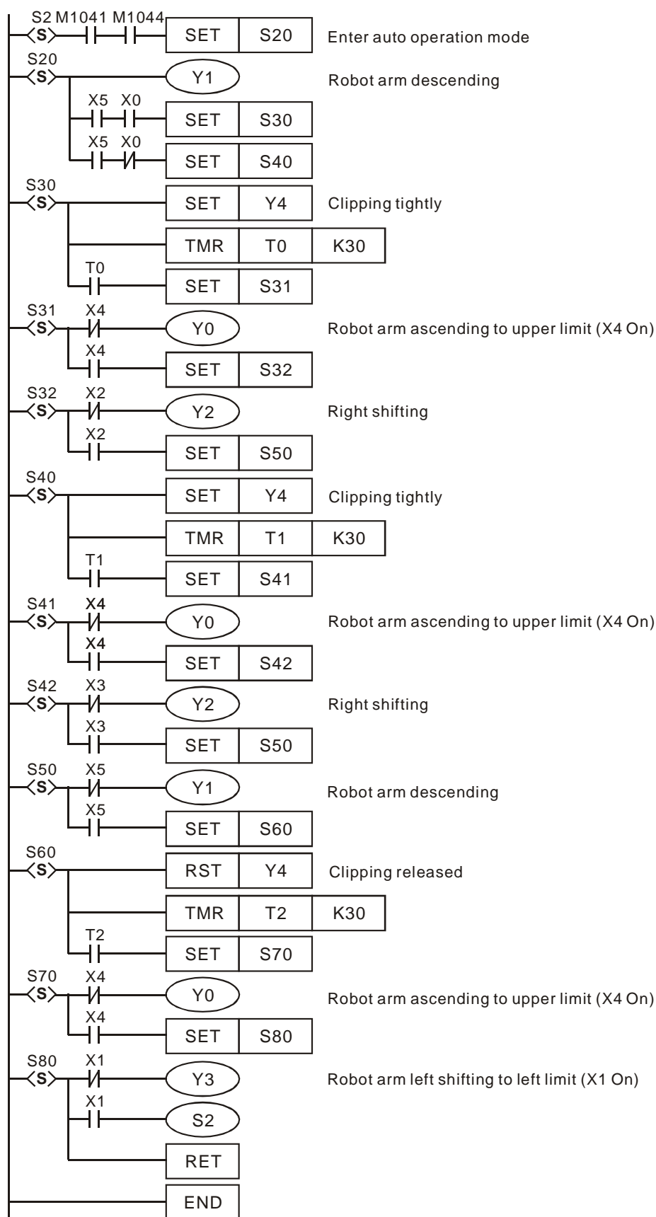
Ladder Diagram:
