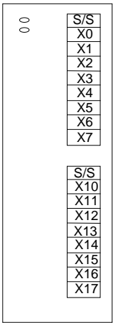
DVP16SM11N
