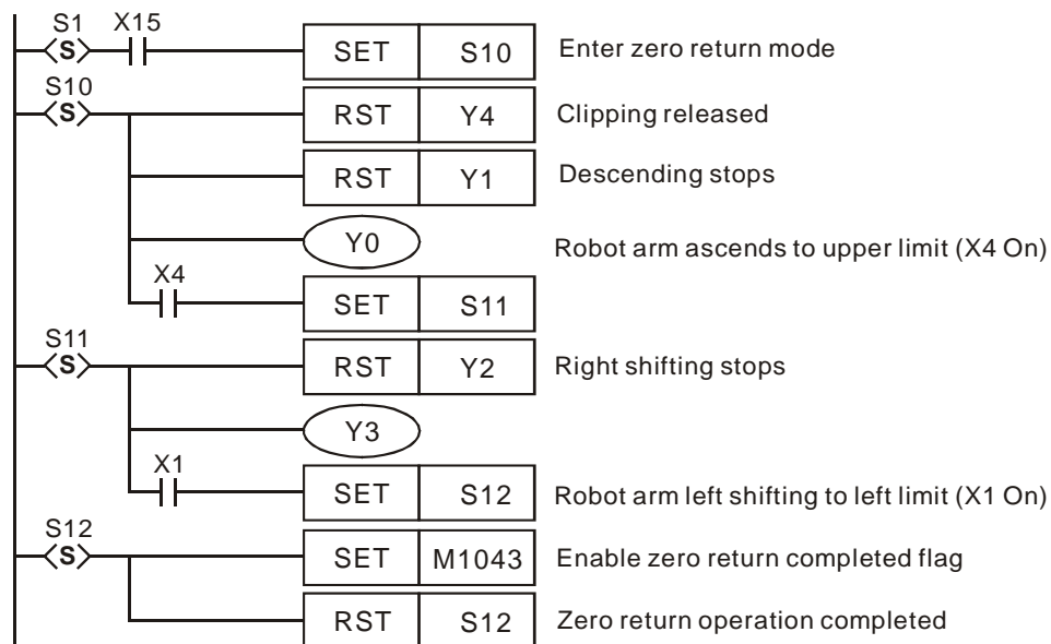
Ladder Diagram:
