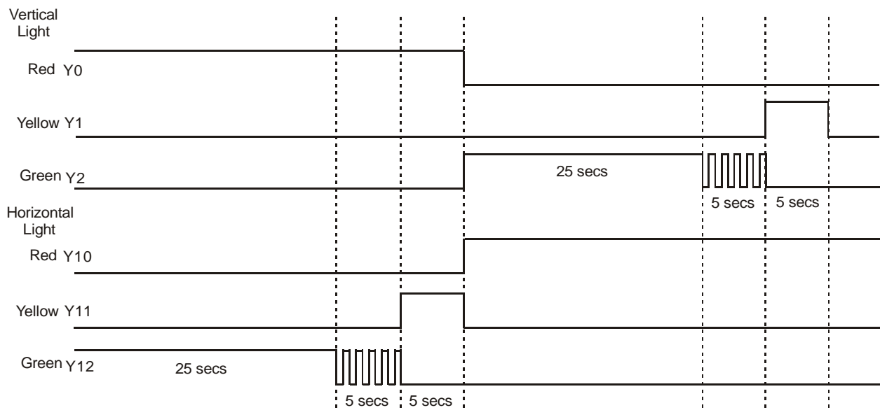
Timing Diagram:
