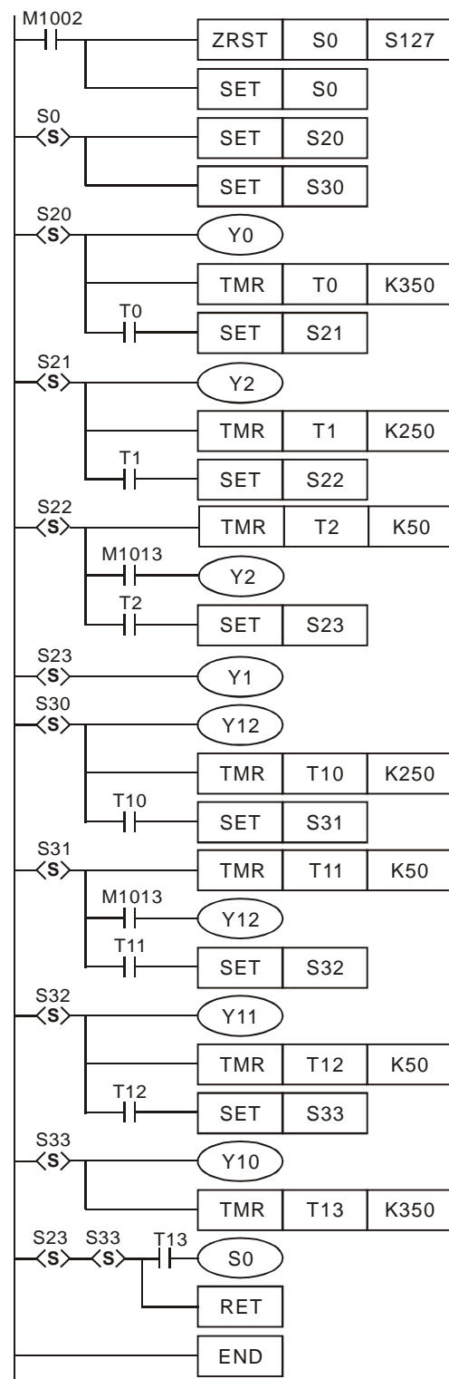
Ladder Diagram:
